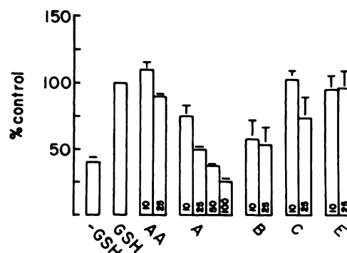
FIG. 5. Effects of purified glutathione S -transferase isozymes on hydrocarbon formation
